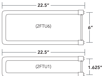
G13 Bi-Pin
